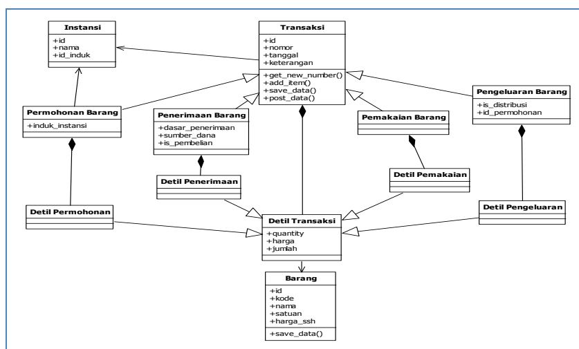
Gambar 4 Class Diagram
