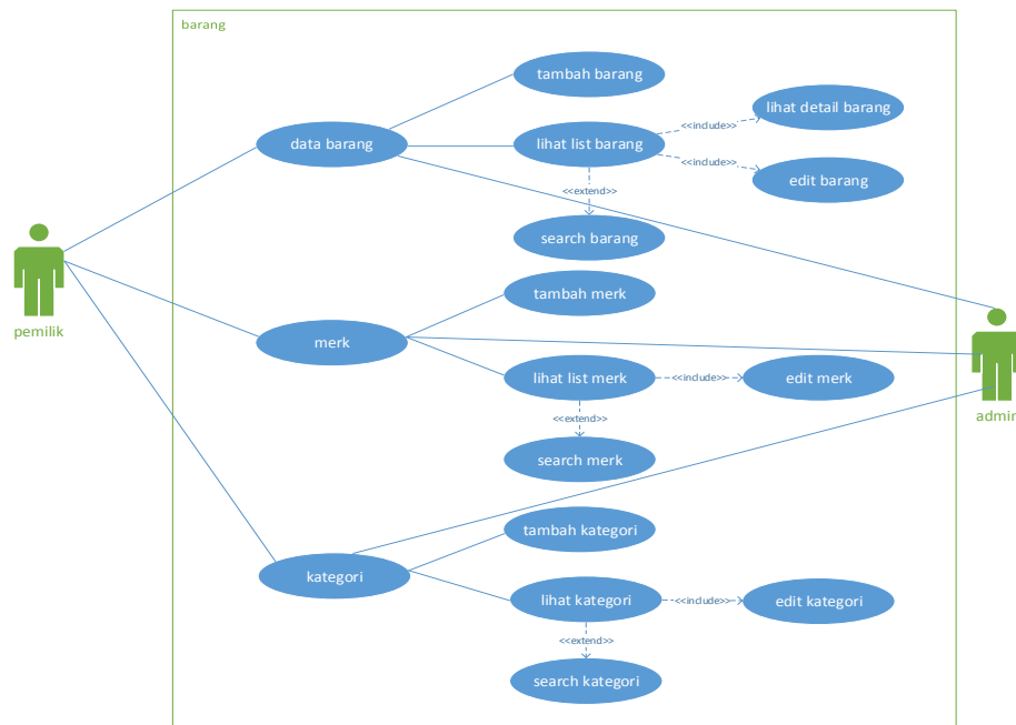
Gambar 6. Use Case Diagram Kelola Barang
