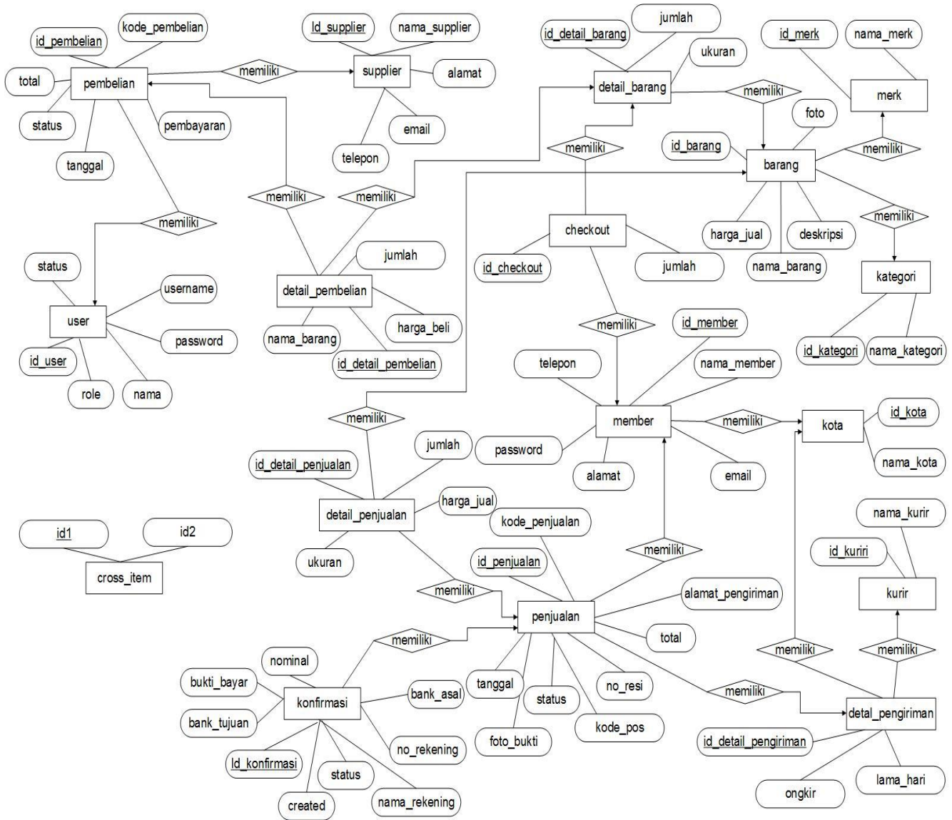
Gambar 2. Gambar Entity Relationship Diagram
