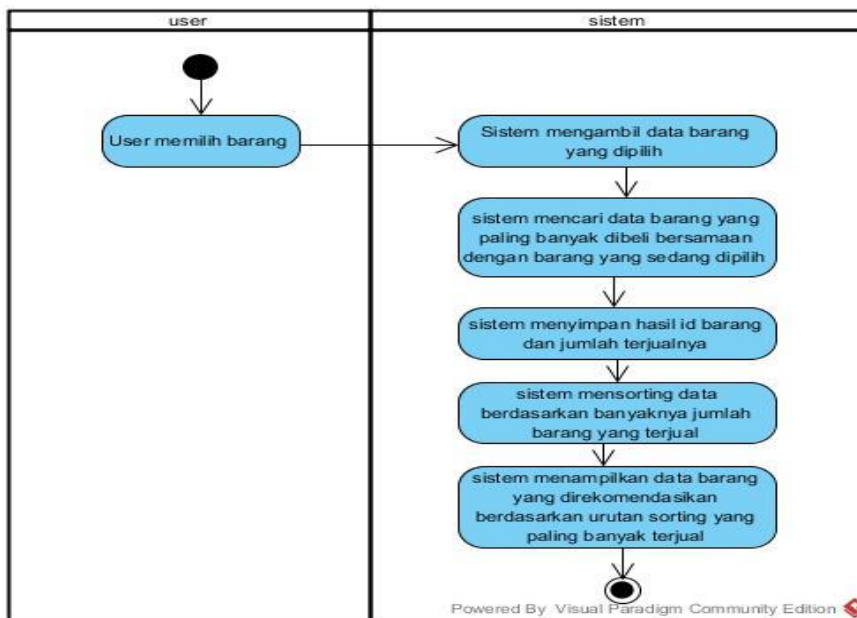
Gambar 8. Activity Diagram Cross Selling
